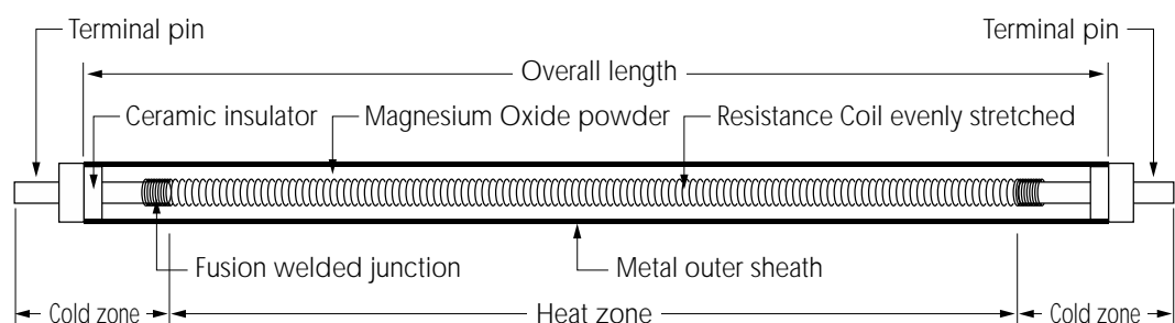
Thermal Tubular-Calrod element construction
