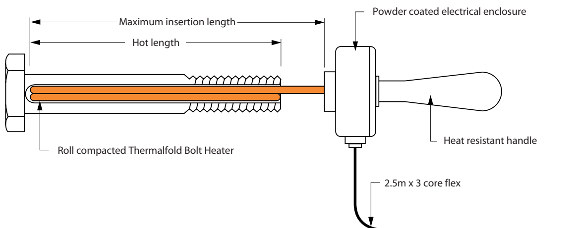
Typical TEE Bolt Heater Design
