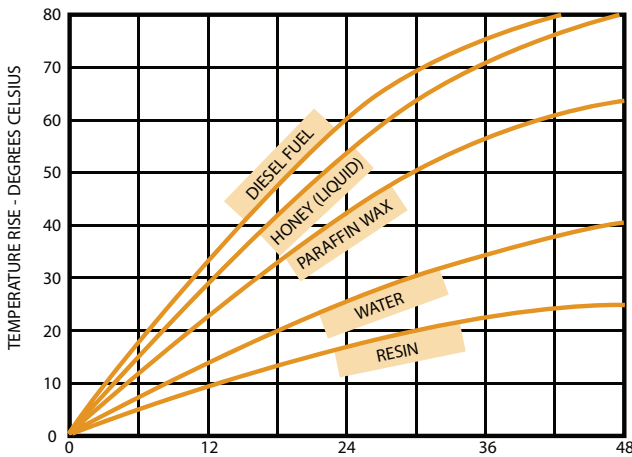
GUIDE TO APPROXIMATE HEATING TIMES FOR 200 LITRE DRUMS OF VARIOUS PRODUCTS AT 15°C AMBIENT
